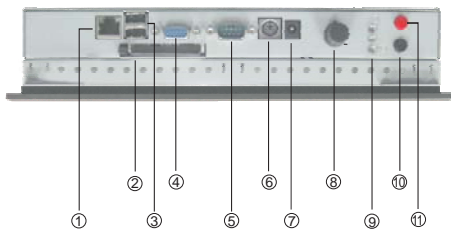
Panel Mount (5mm front bezel)
