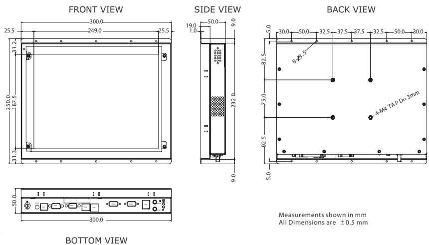
Modularized Construction
