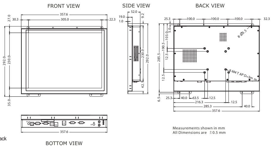
Modularized Construction
