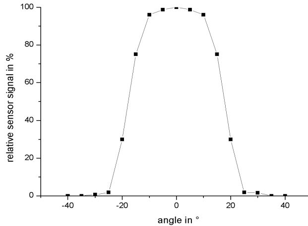
Relative sensor signal depending on the incident angle
