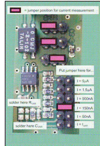
Jumper positions for photodiode input
