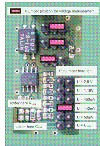
Jumper positions for sensor voltage 0-x Vinput
